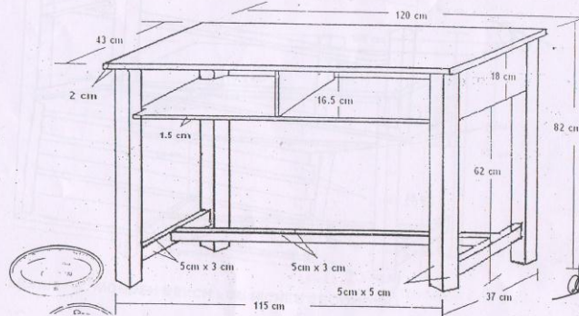
FIGURE - 7. WOODEN DESK FOR HIGHER SECONDARY SECTION
