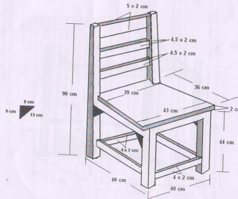
FIGURE - 6 WOODEN CHAIR FOR SECONDARY
