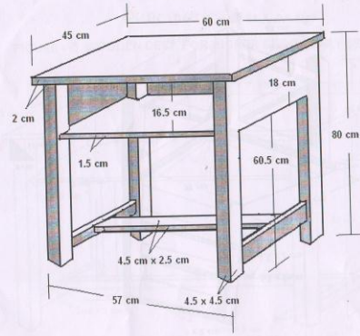
FIGURE - 5. SINGLE WOODEN DESK FOR SECONDARY
