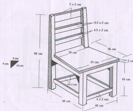
FIGURE - 6 WOODEN CHAIR FOR SECONDARY
