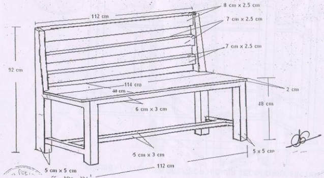
FIGURE - 8. WOODEN BENCH FOR HIGHER SECONDARY
