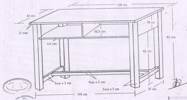
FIGURE - 7. WOODEN DESK FOR HIGHER SECONDARY SECTION
